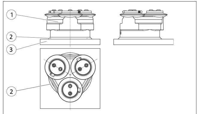
Joint sealing
