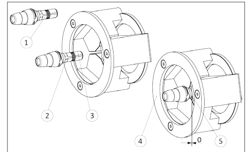
1 Pressure indication 2 Flattened 3 Data Matrix Code 4 SRE 5 Onto stop
